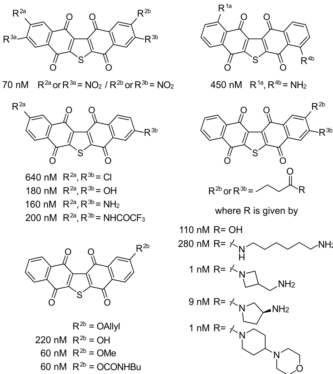
Figure 4. Exemplary analogues of seriniquinone prepared to date. IC 50 values are provided for each compound against Malme-3M cells. Under these conditions, the parent seriniquinone ( R^{1a} – R^{4a} = \text{H} and R^{1b} – R^{4b} = \text{H} ) displayed an IC 50 value of 60 nM.
